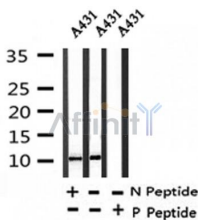
Western blot analysis of Phospho-Histone H4(Ser88) in lysates of A431, using Phospho-Histone H4(Ser88) Ab(AF4358).
