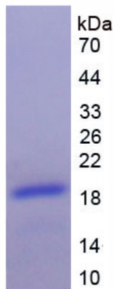
Figure 1. SDS-PAGE
