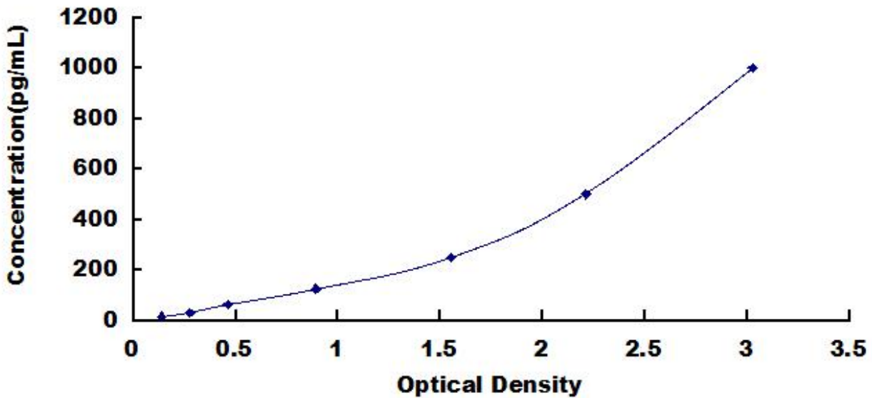
Typical Standard Curve for GPX1, Rat ELISA.
