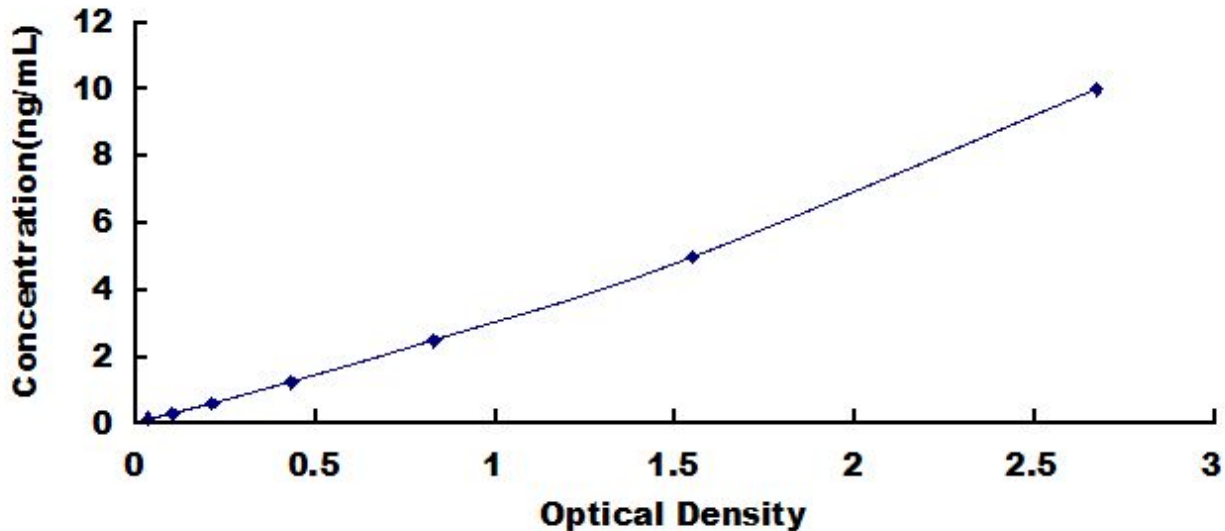
Typical Standard Curve for MIF, Porcine ELISA.
