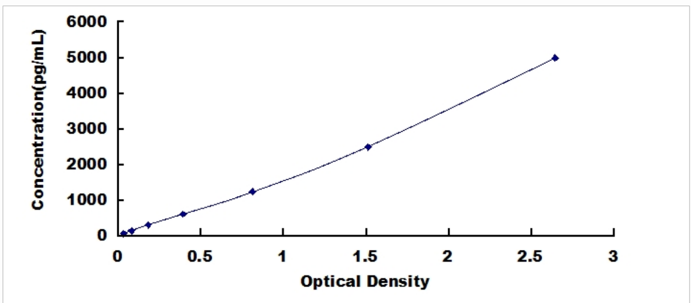
Typical Standard Curve for SLPI, Rat ELISA.
