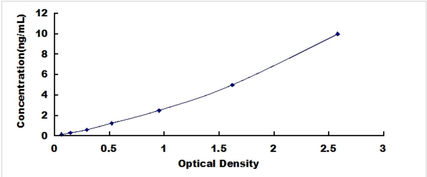
Typical Standard Curve for TSPAN30, Rabbit ELISA.
