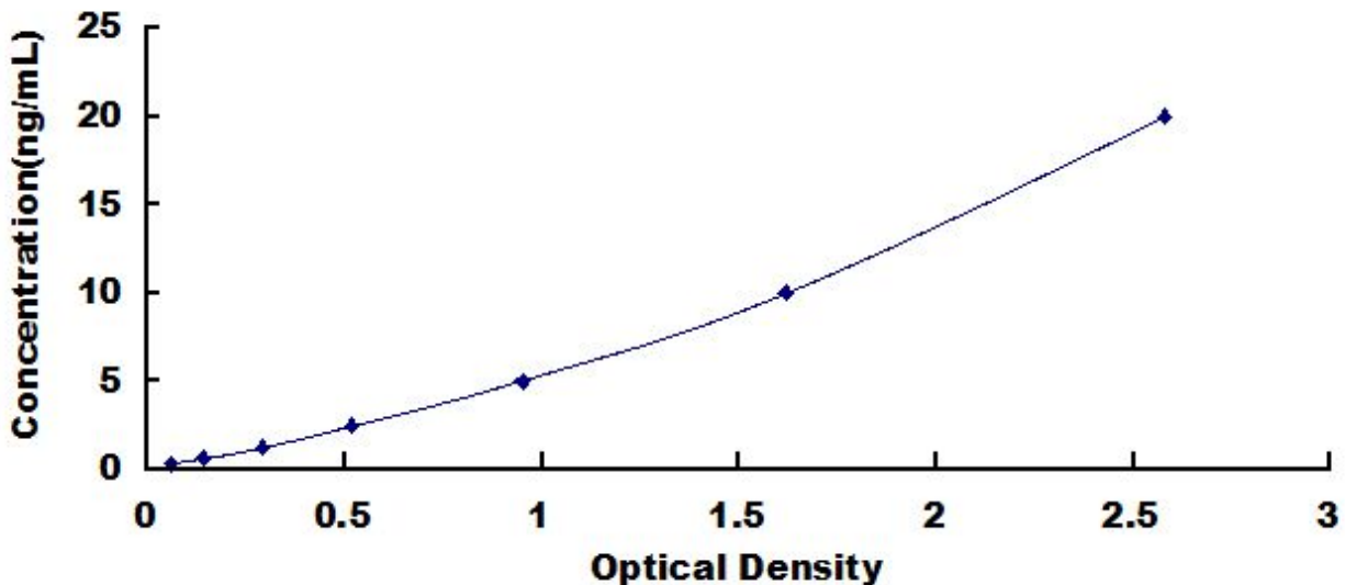
Typical Standard Curve for OAS1, Mouse ELISA.
