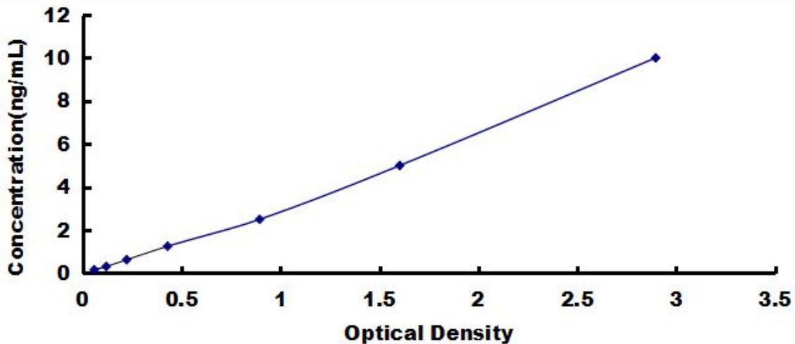
Typical Standard Curve for HTR3A, Human ELISA.
