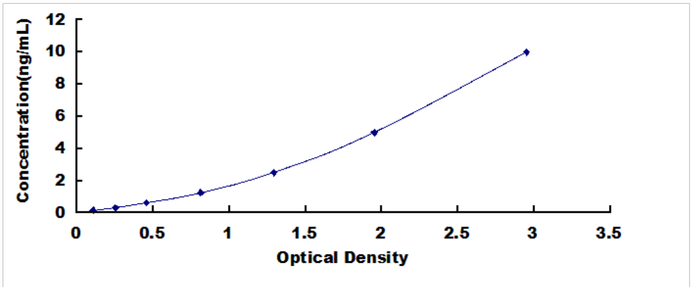
Typical Standard Curve for NT5C, Human ELISA.
