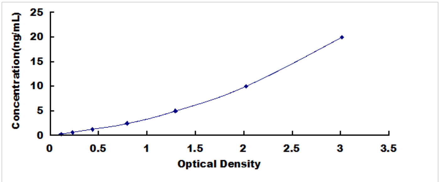
Typical Standard Curve for PGAM1, Mouse ELISA.
