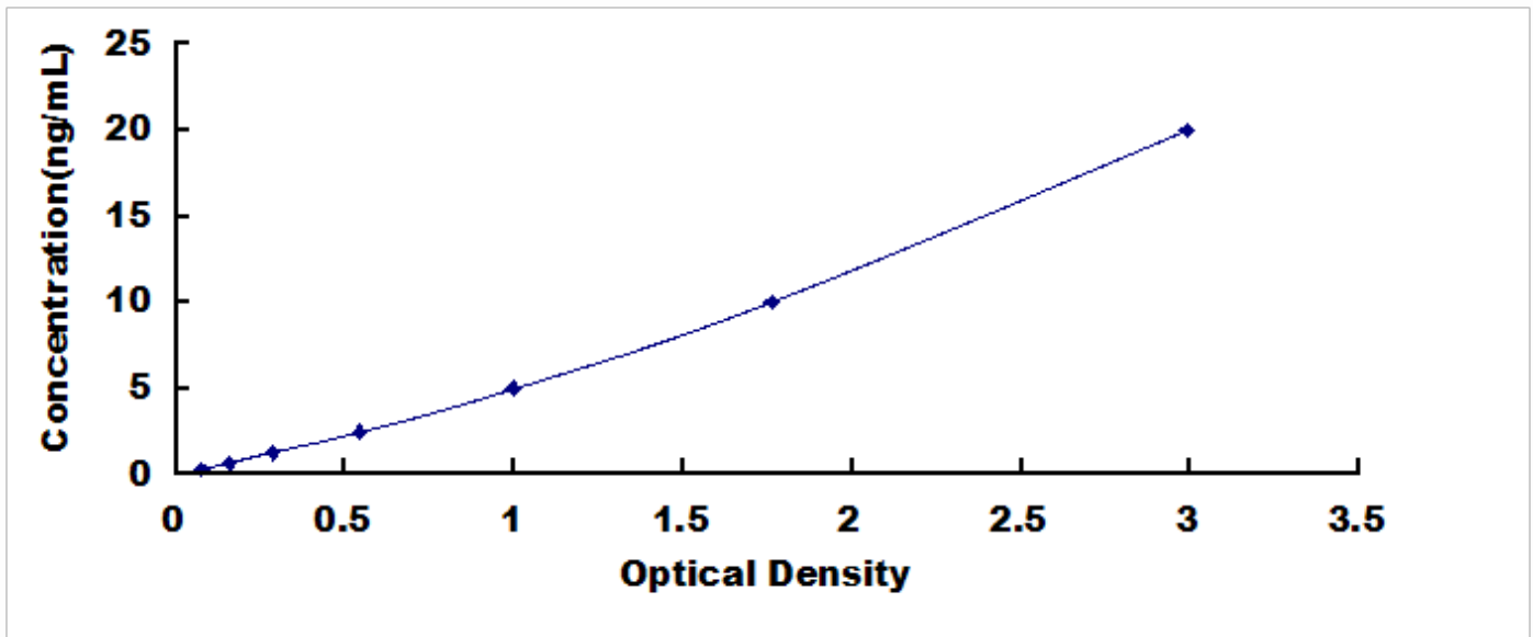
Typical Standard Curve for PGAM1, Rat ELISA.
