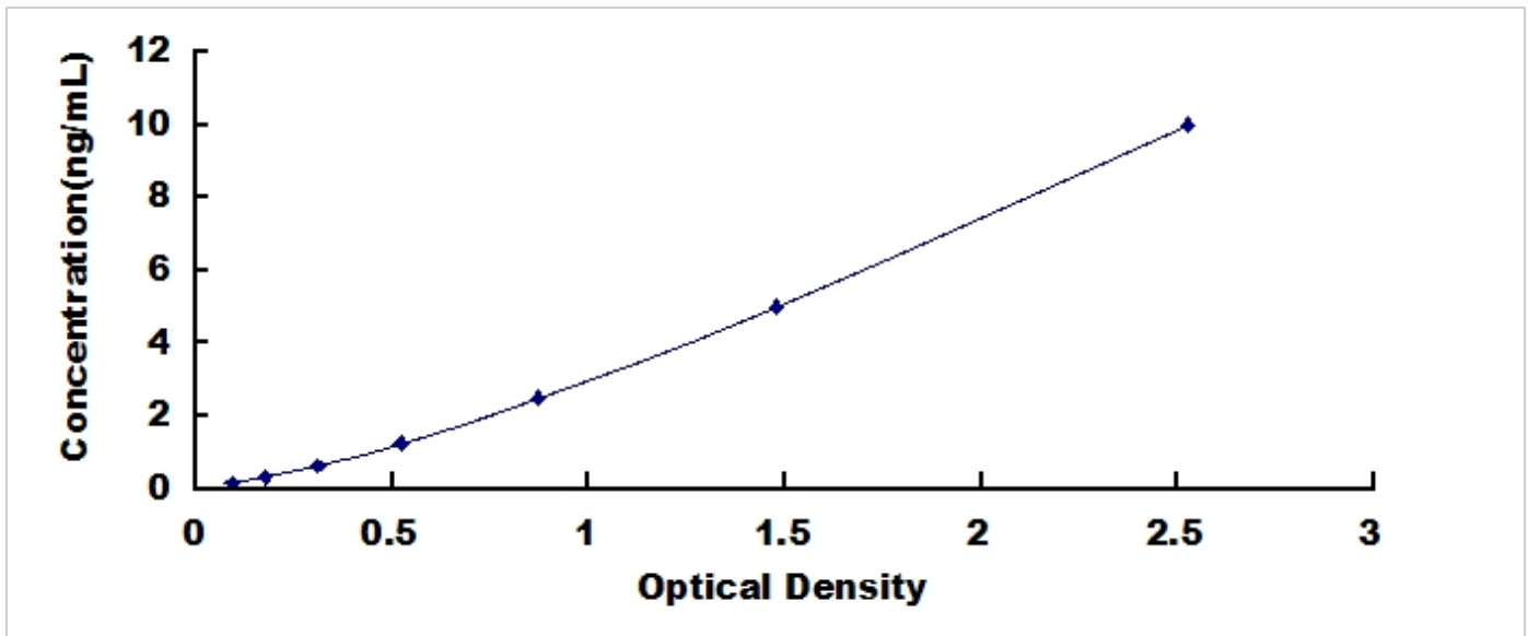
Typical Standard Curve for DNASE1L3, Human ELISA.
