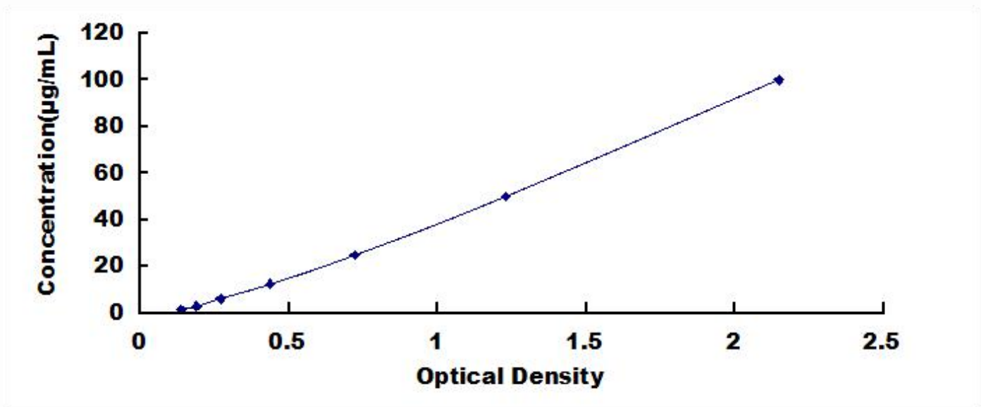
Typical Standard Curve for Creatinine ELISA.
