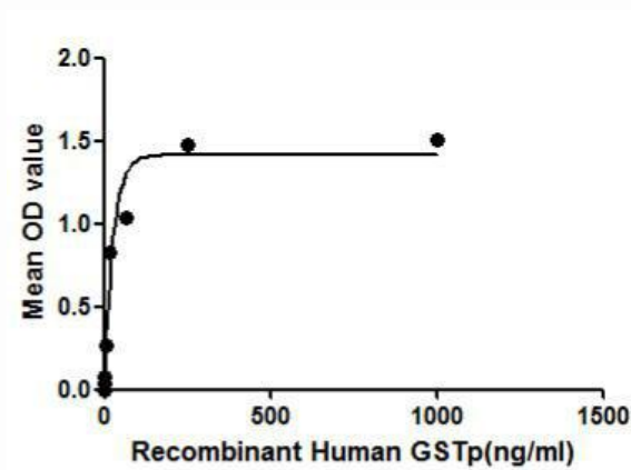
Figure 1. The binding activity of GSTp with CDK5.
