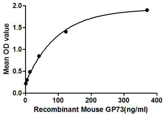
Figure 1. The binding activity of GP73 with DYM.
