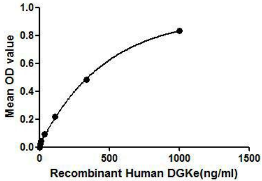
Figure 1. The binding activity of DGKe with PDHA.
