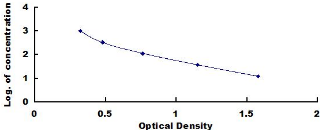
Typical Standard Curve for Adrenomedullin, Human ELISA.
