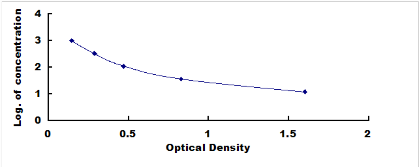
Typical Standard Curve for Adrenomedullin, Rat ELISA.
