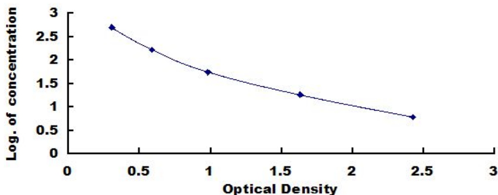
Typical Standard Curve for TRH, Human ELISA.
