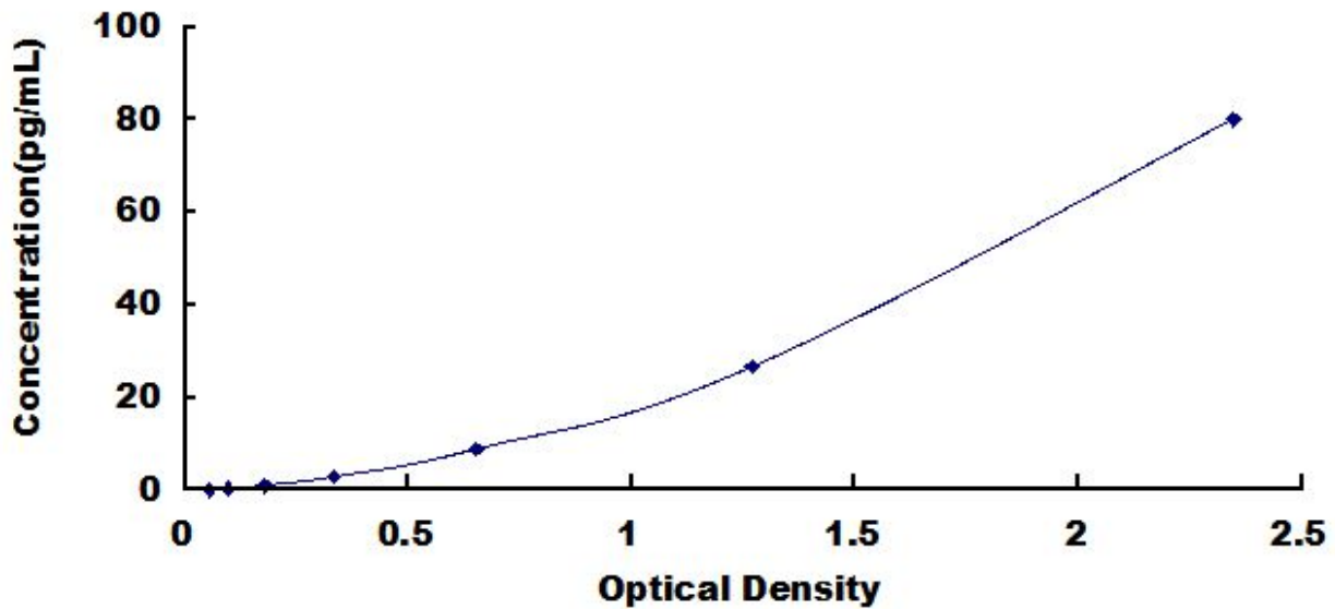
Typical Standard Curve for F1+2, Human ELISA.
