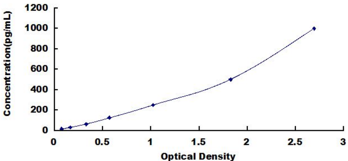
Typical Standard Curve for Uromodulin, Human ELISA.
