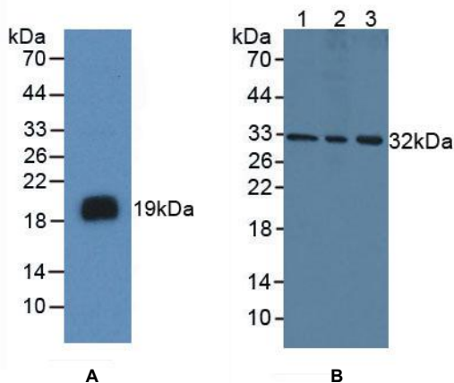
Figure 1. Western Blot
