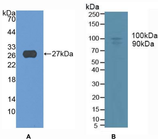
Figure 1. Western Blot
