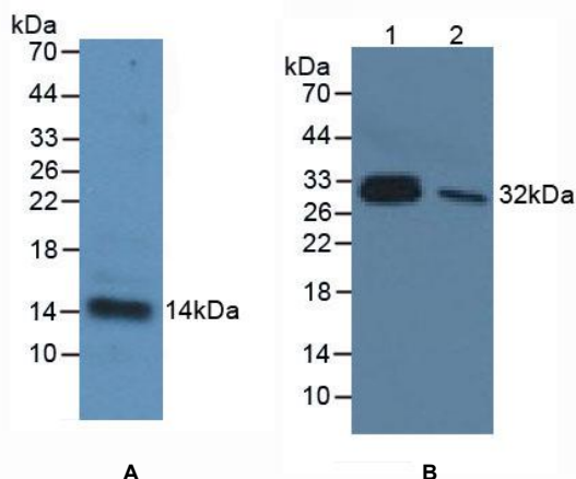
Figure 1. Western Blot
