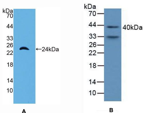
Figure 1. Western Blot
