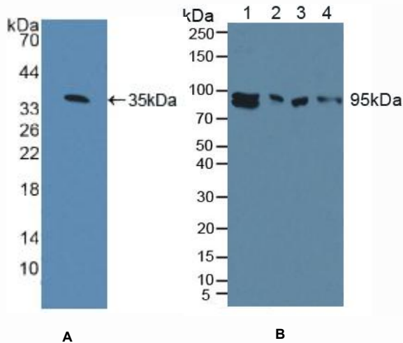
Figure 1. Western Blot
