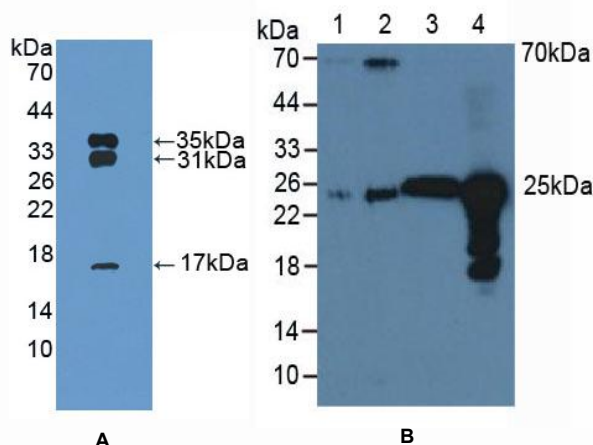
Figure 1. Western Blot
