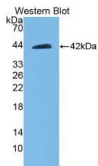
Figure 1. Western Blot; Sample: Recombinant BECN1, Rat.
