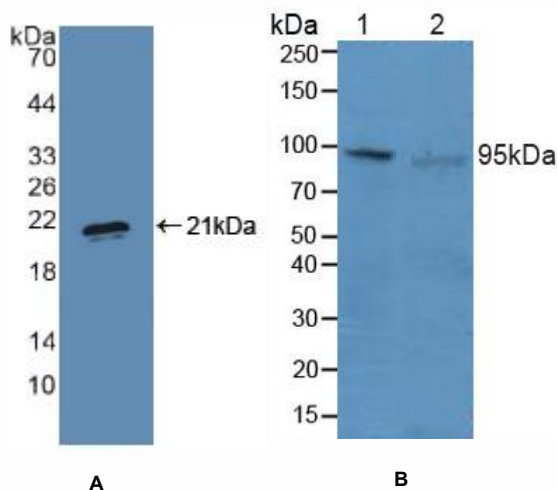
Figure 1. Western Blot
