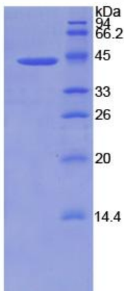
Figure 2. SDS-PAGE
