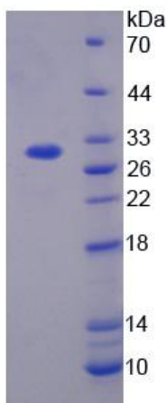
Figure 1. SDS-PAGE
