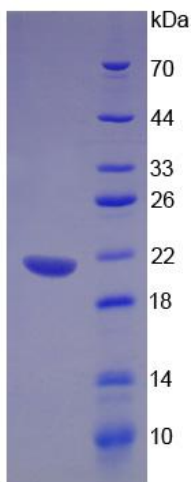
Figure 1. SDS-PAGE
