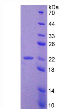
Figure 2. SDS-PAGE
