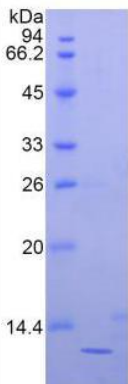
Figure 2. SDS-PAGE
