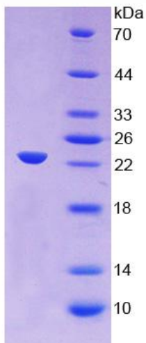
Figure 2. SDS-PAGE
