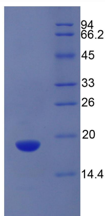
Figure 1. SDS-PAGE
