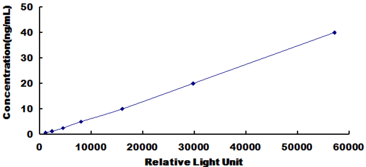
Typical Standard Curve for Mouse AGT CLIA.
