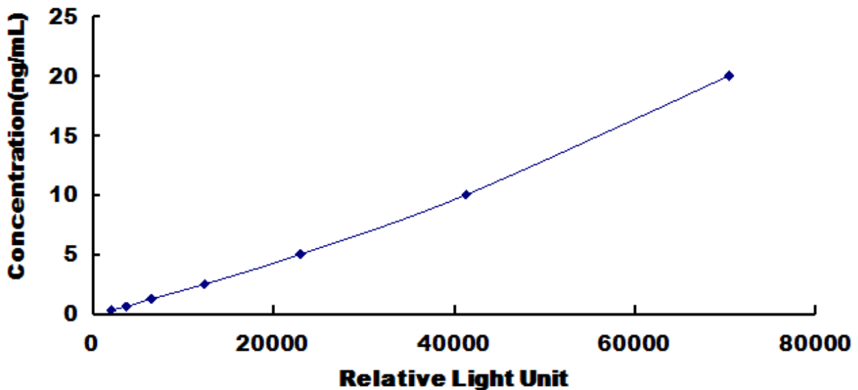
Typical Standard Curve for Human VS CLIA.
