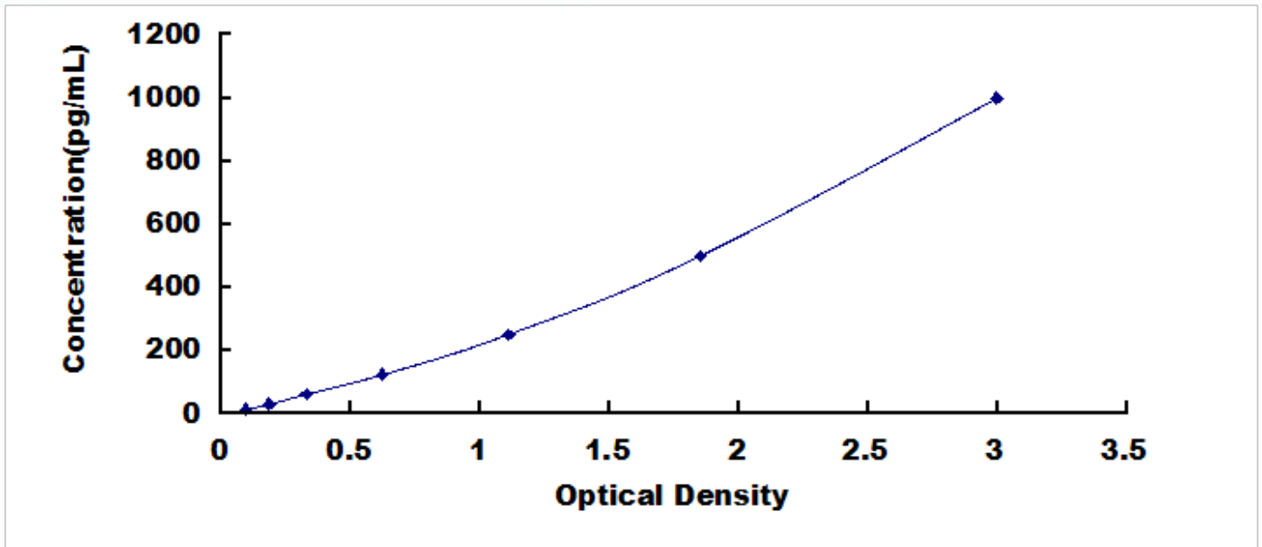
Typical Standard Curve for BMP2, Rat ELISA.
