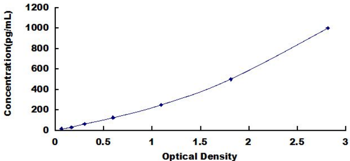
Typical Standard Curve for VEGFD, Mouse ELISA.
