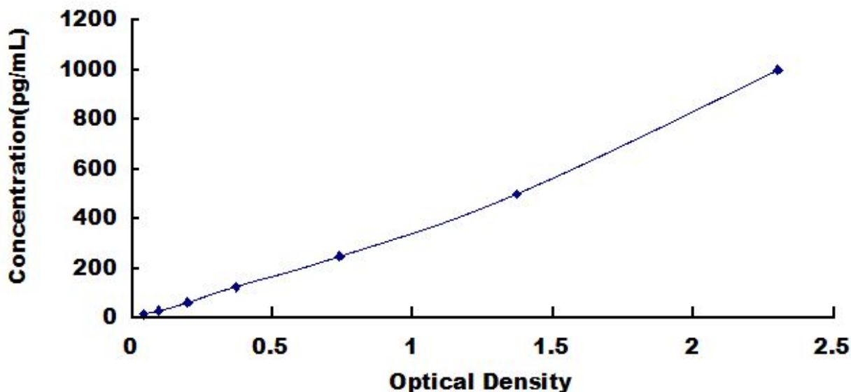
Typical Standard Curve for INHA, Rat ELISA.
