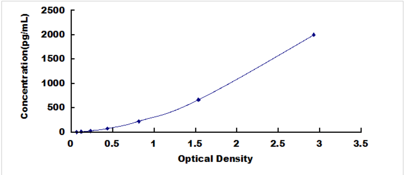
Typical Standard Curve for BNP, Human ELISA.
