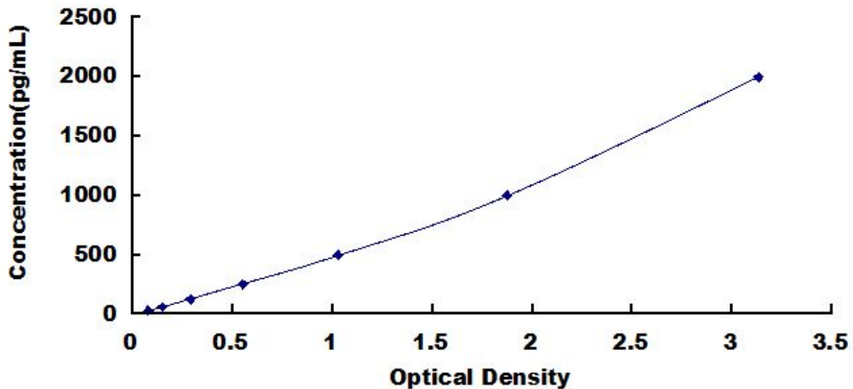
Typical Standard Curve for SPD, Mouse ELISA.
