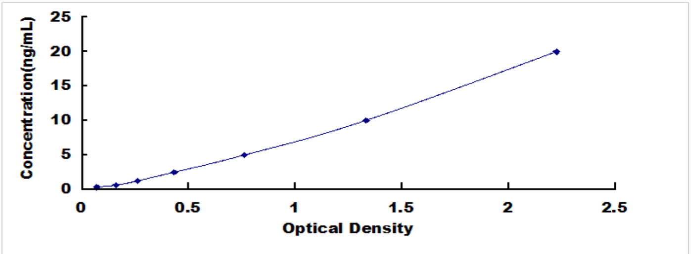
Typical Standard Curve for PLA2G2D, Human ELISA.
