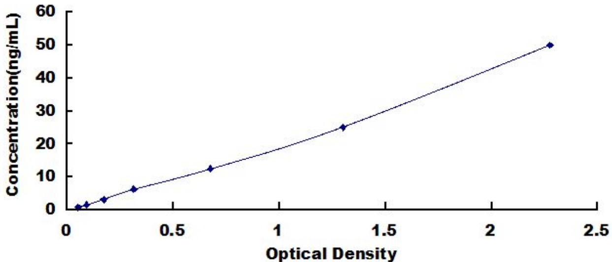
Typical Standard Curve for Bax, Human ELISA.
