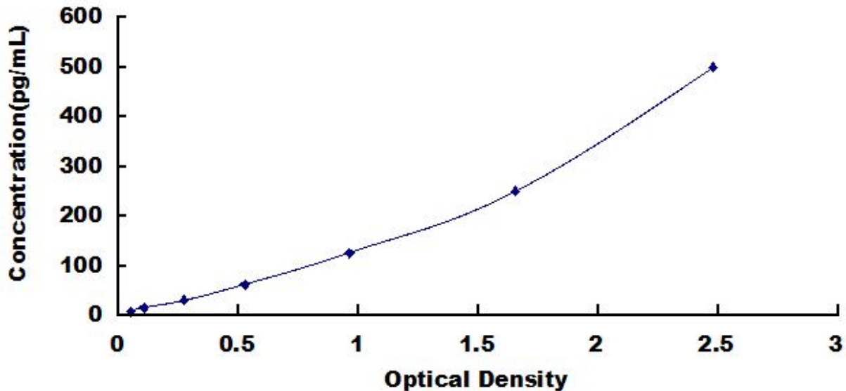
Typical Standard Curve for IL35, Mouse ELISA.
