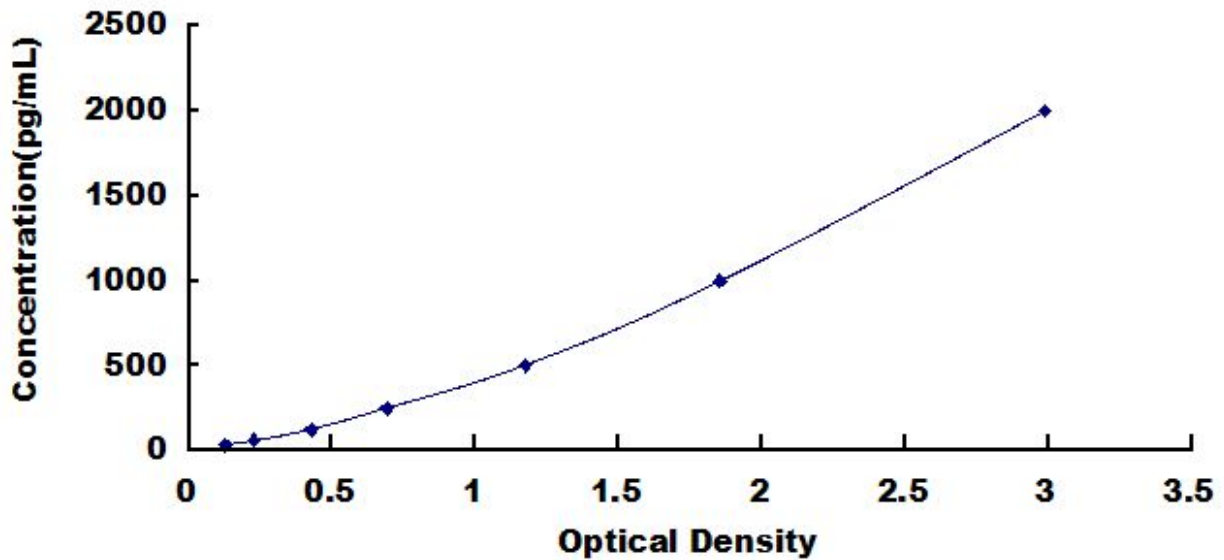
Typical Standard Curve for C5b-9, Rat ELISA.
