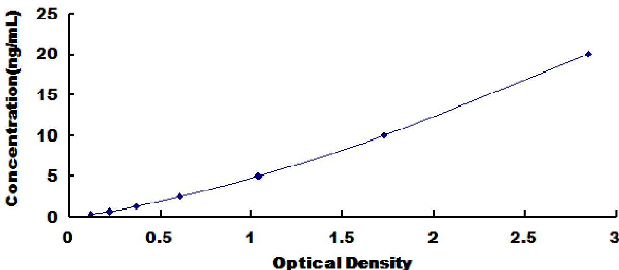
Typical Standard Curve for PFKM, Human ELISA.
