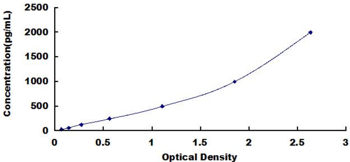
Typical Standard Curve for PRDX2, Human ELISA.
