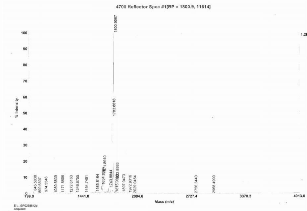
Figure 2. MASS Spectrometry
